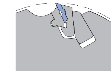
Lightweight aluminium tool body with steel chip breaker
