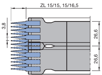
Minifinger joint cutter ZL 15 mm, TG 3.8 mm
