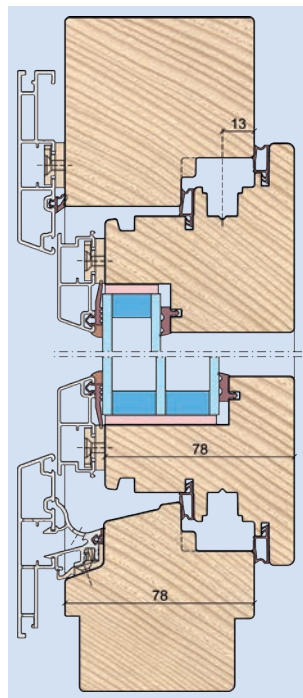
IV78 ClimaTrend 13 mm gear axle
